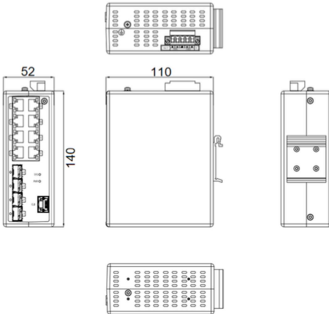
ISM7312D (52 × 140 × 110 mm)
